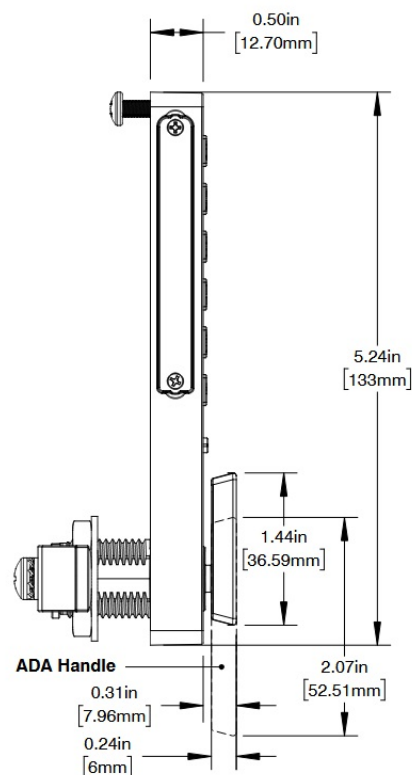
SIDE VIEW
