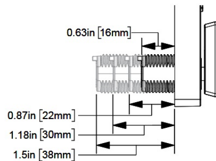
CYLINDER LENGTH
