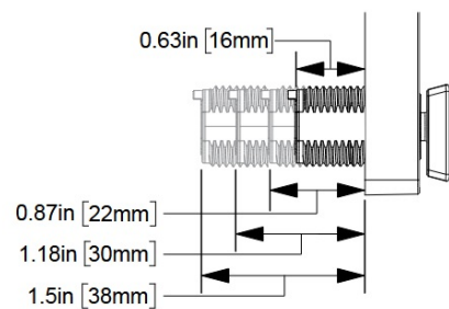
CYLINDER LENGTH
