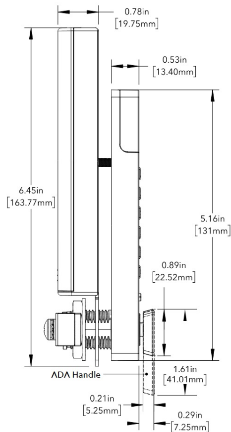
SIDE VIEW
