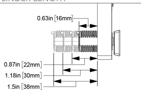
CYLINDER LENGTH
