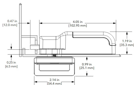
Top View-Pin Connector
