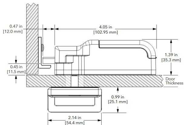
Top View-Cable
