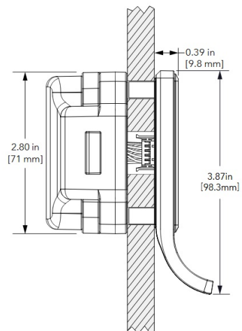
Side View-Cable
