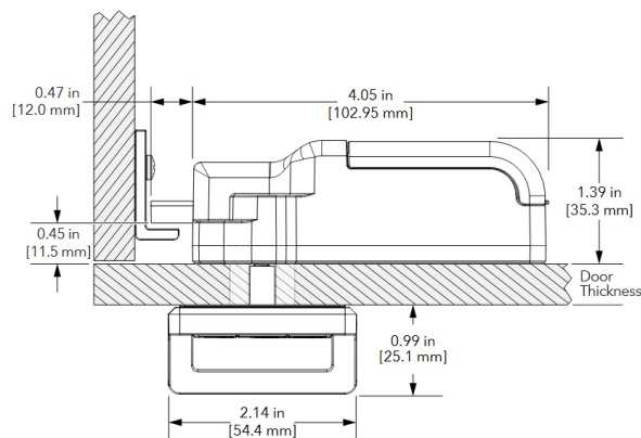
Top View-Cable
