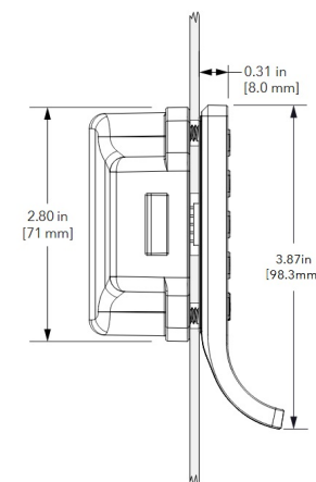
Side View-Pin Connector
