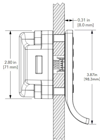
Side View-Cable
