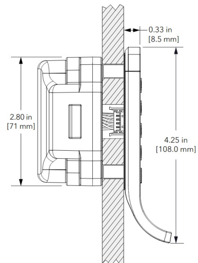
Side View-Cable
