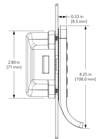
Side View-Pin Connector
