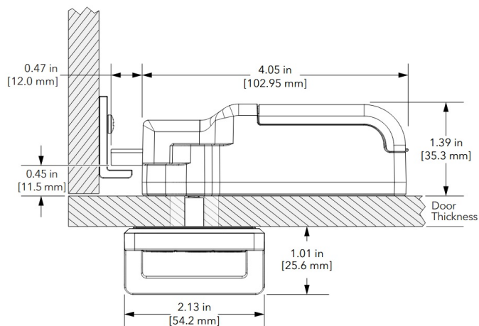
Top View-Cable
