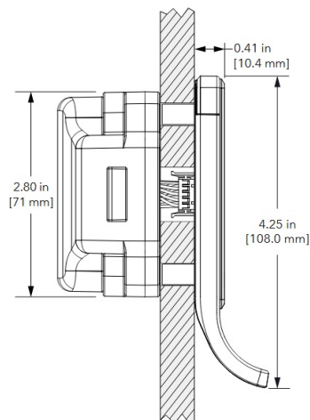
Side View-Cable
