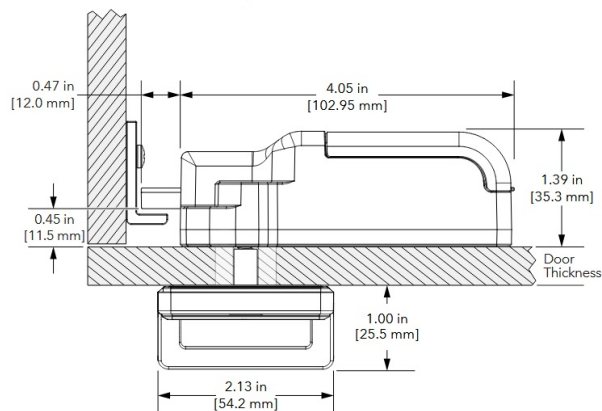
Top View-Cable
